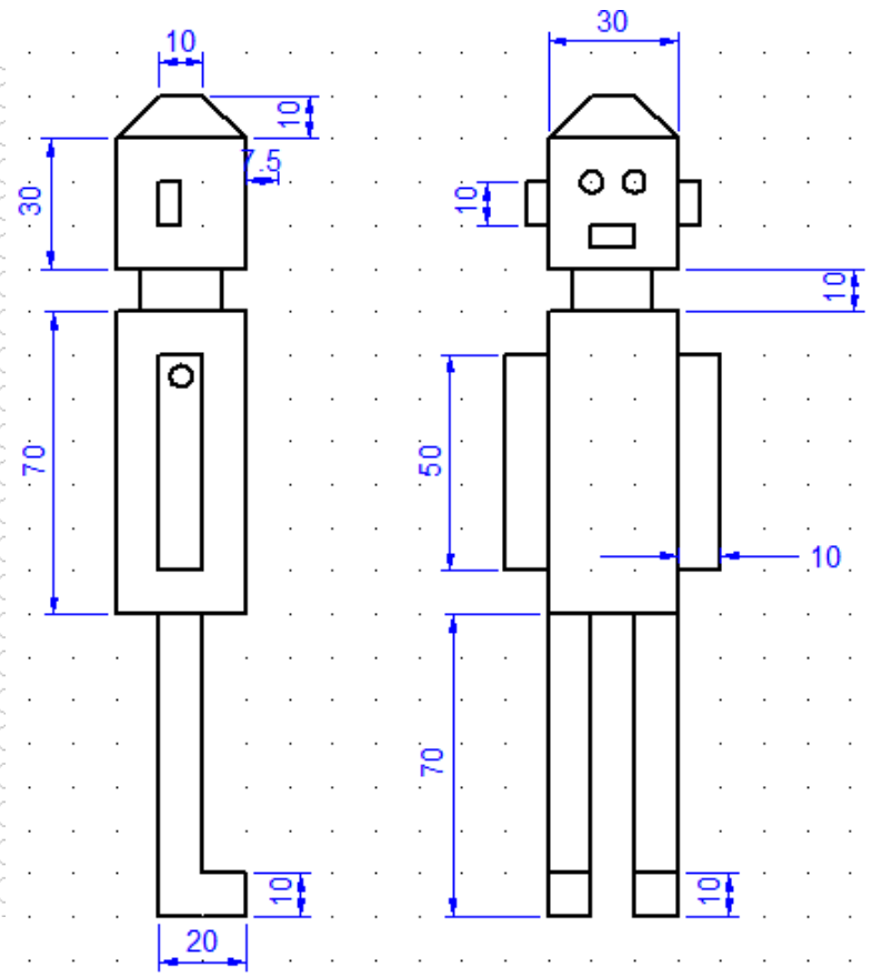
Orthogonal Grid – 10mm
